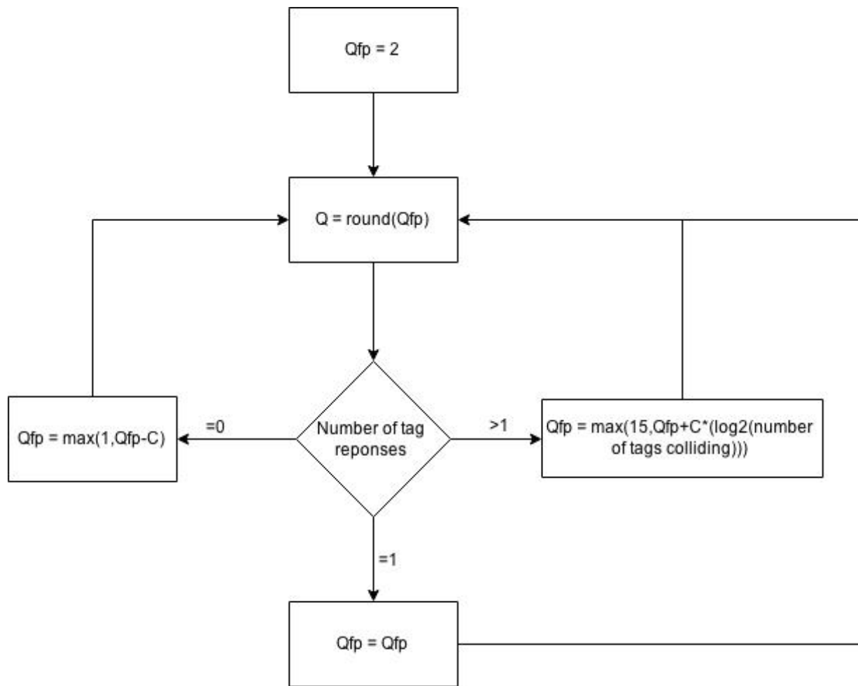
Figure 4.5: Algorithm for choosing the value of Q parameter in QSCC algorithm
